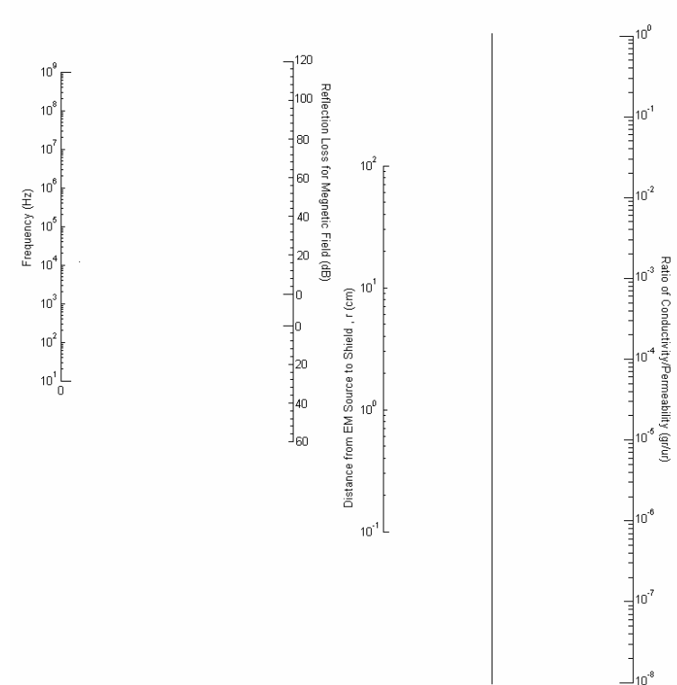
Figure 2a. Reflection Loss Nomograph for Magnetic Field
